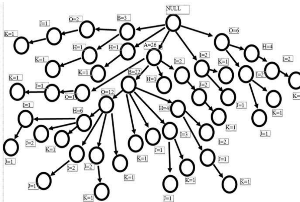
Figure 3. Result of FP-tree Formation After TID 39
